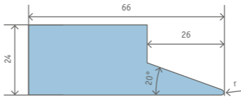
SCHARFSCHIENE 66/24 20°
