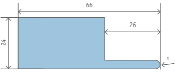
RUNDSCHIENE 66/24 R = 1 - 12
